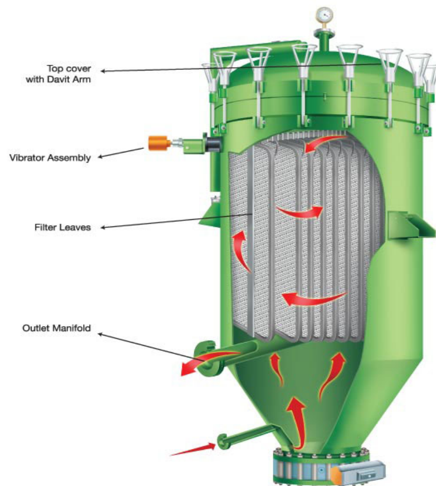
Vertical Pressure Leaf Filter
